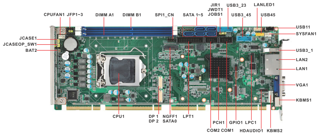
Figure 1.1 Jumper and connector locations
