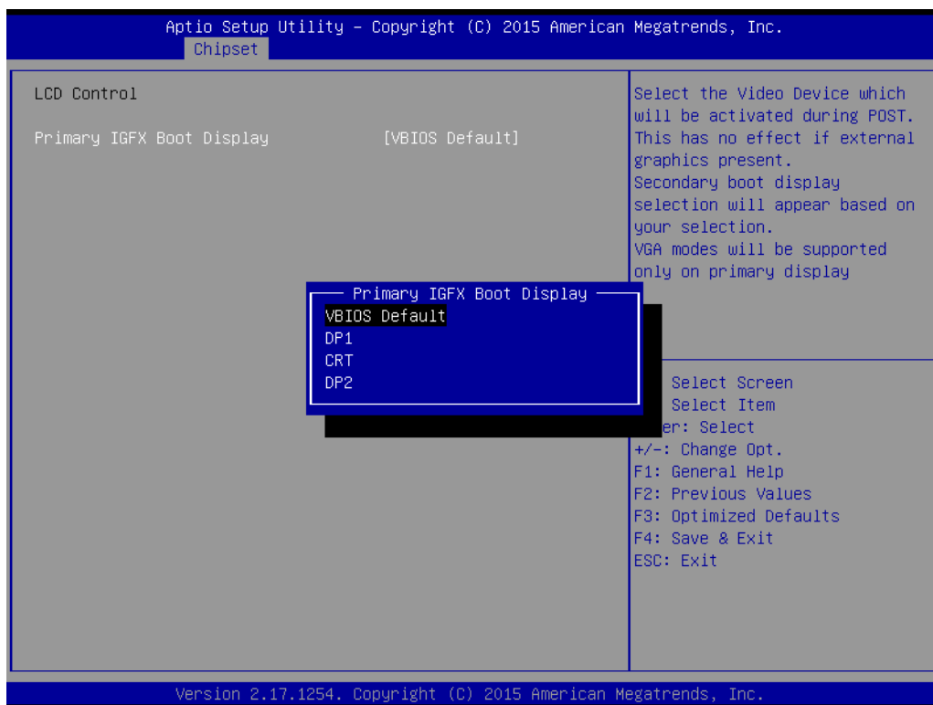
Figure 3.23 Graphics Configuration
