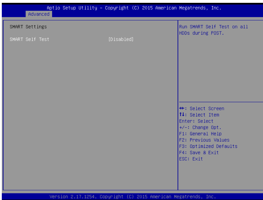
Figure 3.8 Smart Setting
