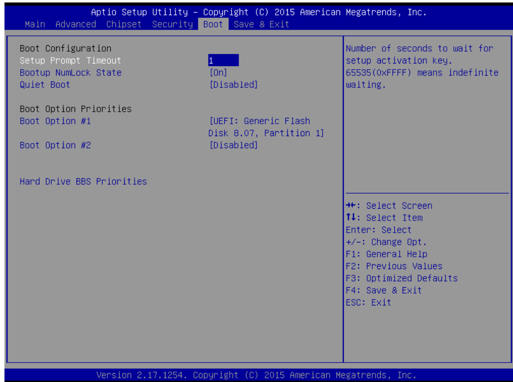
Figure 3.31 Boot
