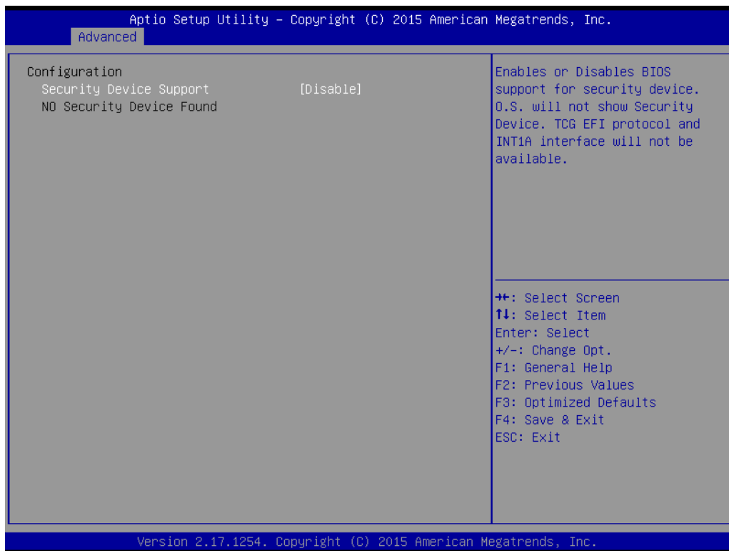
Figure 3.4 Trust Computing
