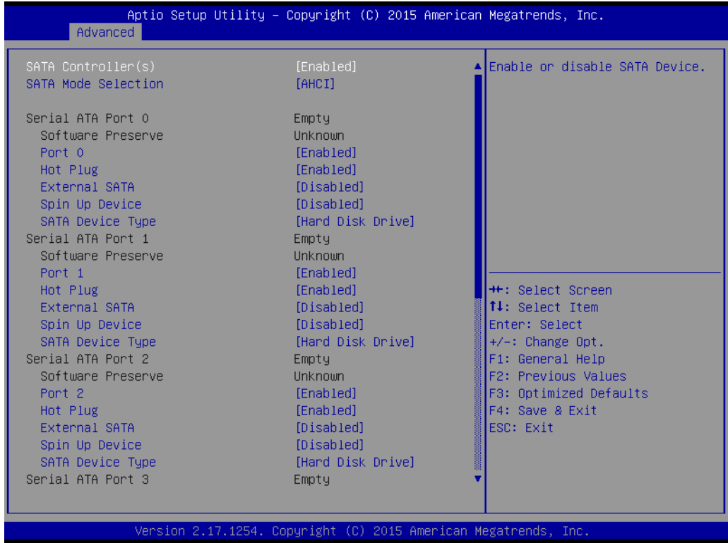
Figure 3.17 SATA Configuration
