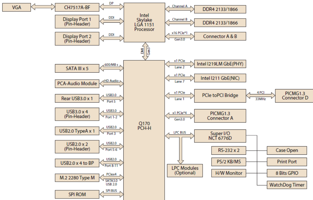
Figure 1.3 PCE-5129 block diagram
