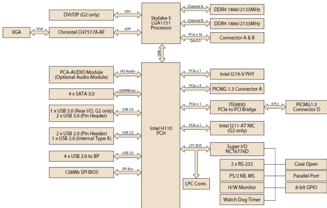
Figure 1.4 PCE-5029 block diagram
