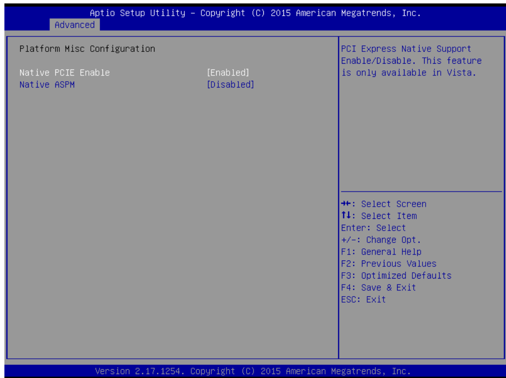
Figure 3.16 Platform Misc Configuration
