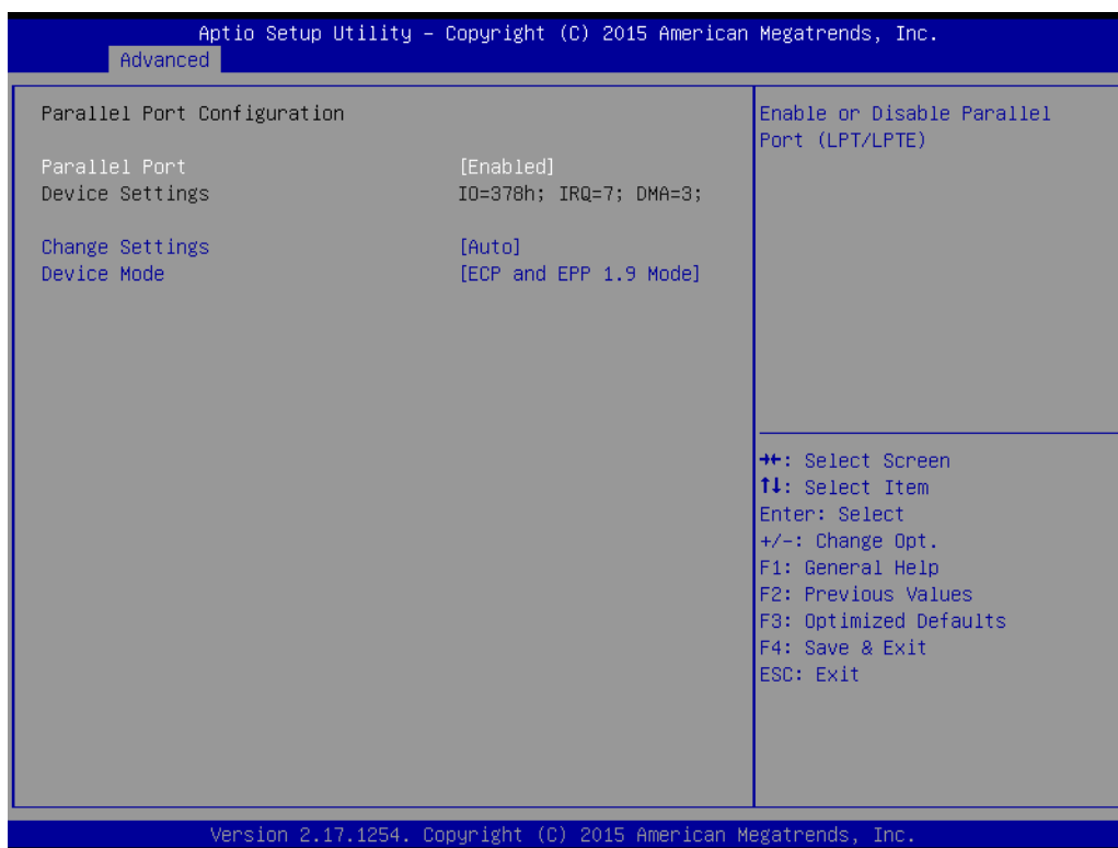
Figure 3.11 Parallel Configuration
