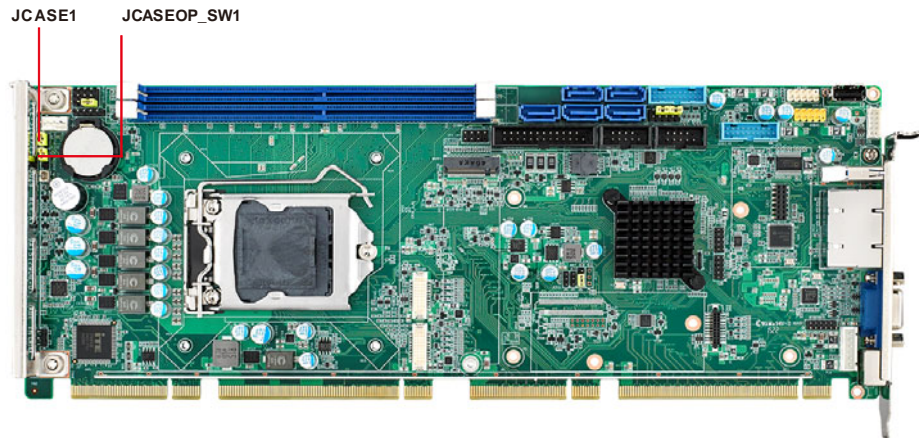
Figure 2.1 Case Open Jumper Locations
