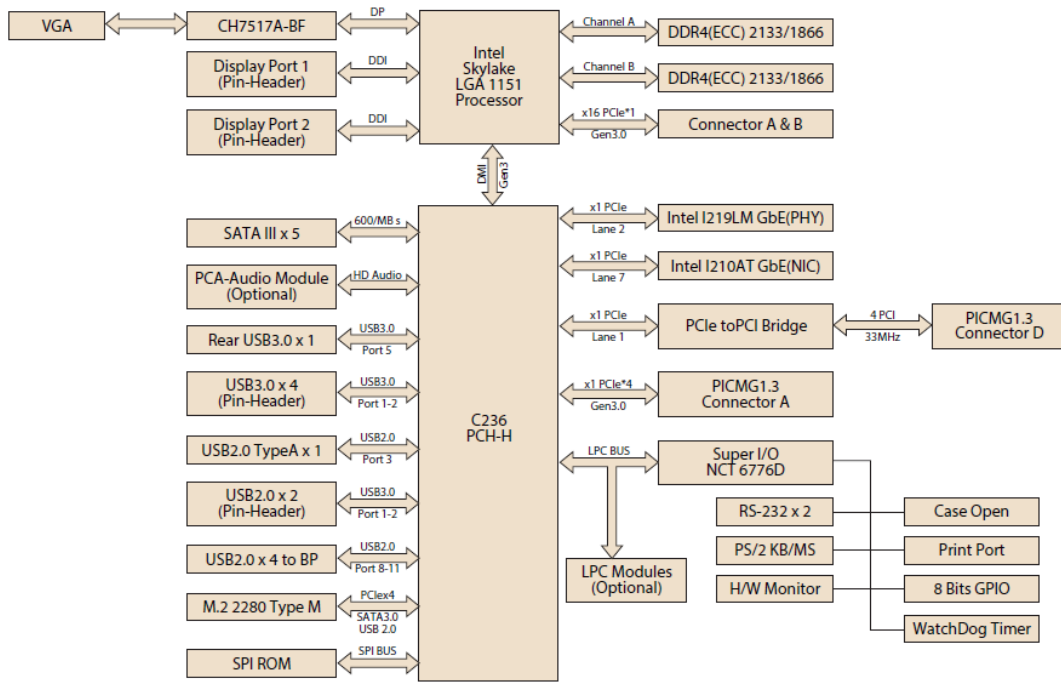
Figure 1.2 PCE-7129 block diagram
