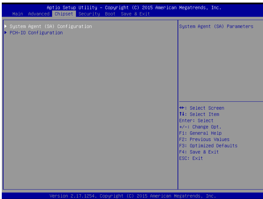
Figure 3.21 Chipset
