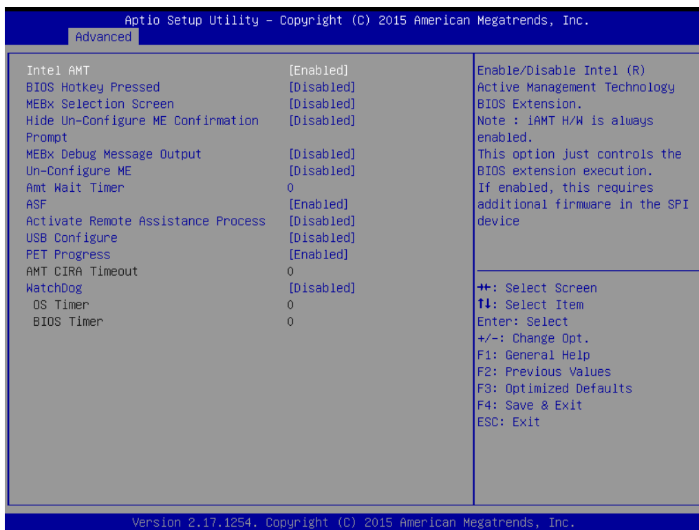
Figure 3.6 AMT Configuration
