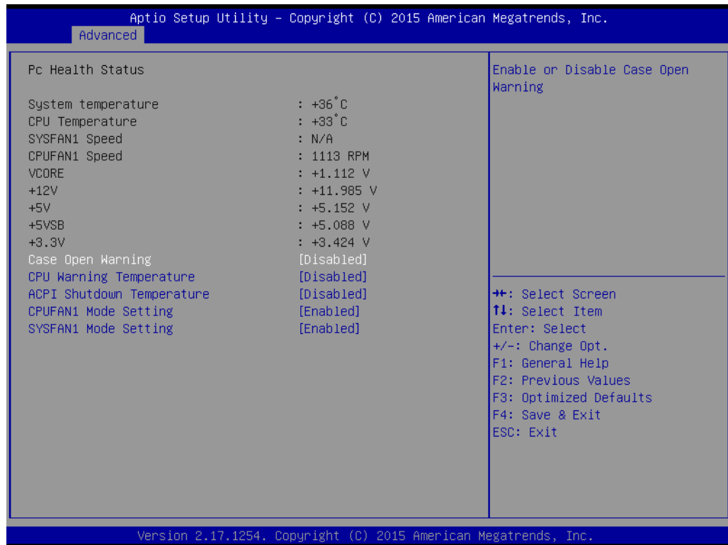
Figure 3.12 PC Health Status
